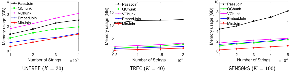
Figure 12: A comparison on memory usage, varying n .
