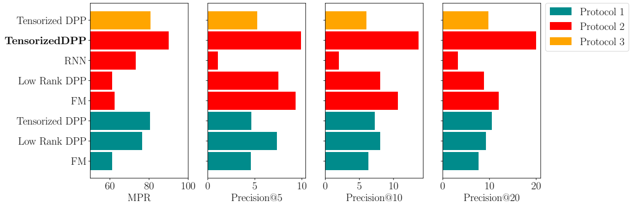
Figure 2: [Ordered Baskets] Performance of the models on Instacart dataset for the three protocols. Protocols 1, 2, and 3 correspond to predicting a randomly removed item, predicting the last added item with last-item removal in the training set (for the tensorized DPP), and predicting the last added item in the test set with random item removal in the training set, respectively. By cross-validation, all models used 80 latent factors, except FM, which used 5 latent factors. The best performance is achieved with our tensorized DPP model, particularly in protocol 2, when involves predicting the last added item; this protocol is the closest to a real-world application.
