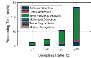
Figure 17. Computation overhead.
