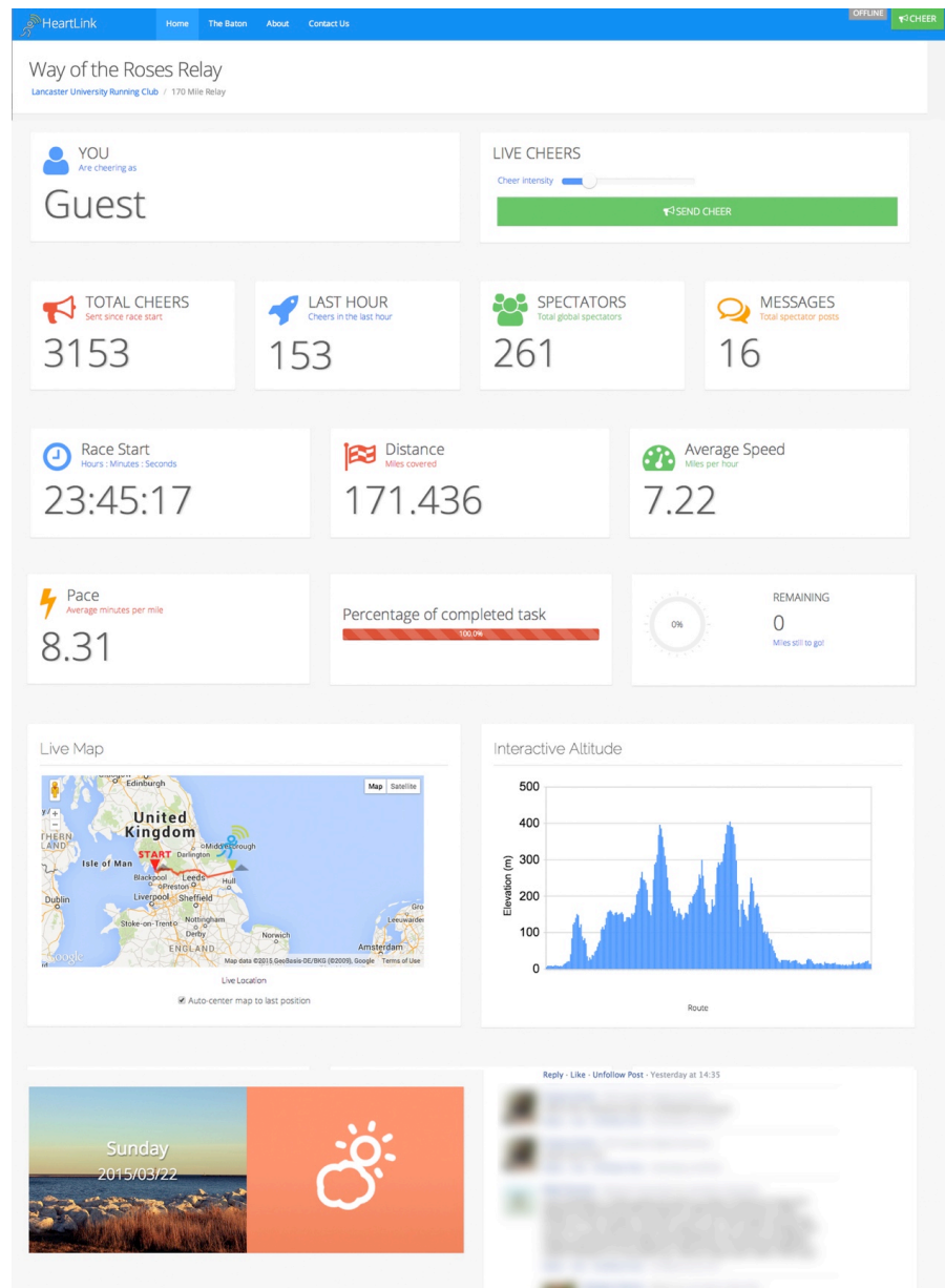
Figure 5: Spectators' interface
