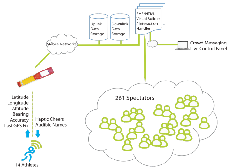
Figure 4: System design
