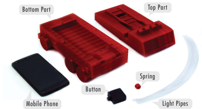
Figure 3. The components of the complete firetruck model.
