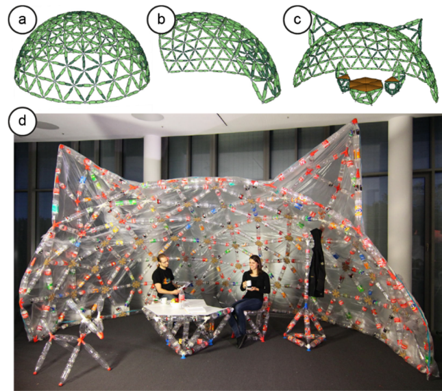
Figure 13: (a) Dome created using the dome tool. (b) We make the opening using the delete tool, and (c) add decoration using the triangle and line tools. (d) The resulting dome is built using 512 bottles.
