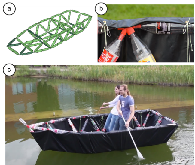
Figure 7: A functional boat created using TrussFab. (a) Using the editor, users can design their structures efficiently. (b) The bottle-frame is simply covered by tarp. (c) The fabricated boat seats two.
