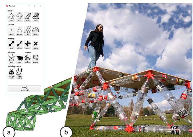
Figure 1: TrussFab is a system that allows users to fabricate large structures sturdy enough to carry human weight. TrussFab considers bottles as beams that form structurally sound node-link structures also known as trusses , allowing it to handle the forces resulting from scale and load.
