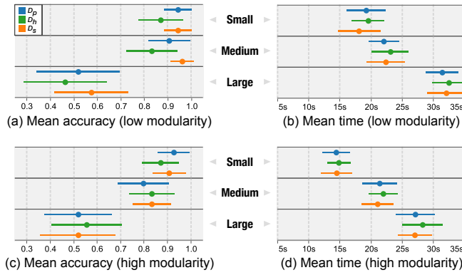
Figure 6. Node exploration task (T1) results of Study I . Error bars represent 95% confidence intervals (CIs).
