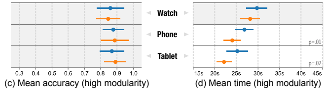
Figure 12. Path exploration task (T3) results of Study II. Error bars represent 95% CIs. Significant rows are highlighted in a white background.
