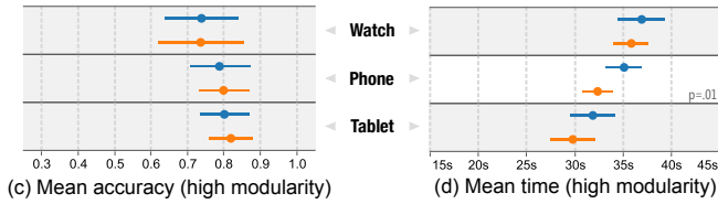
Figure 11. Link exploration task (T2) results of Study II. Error bars are 95% CIs. Rows with significant results are in a white background.
