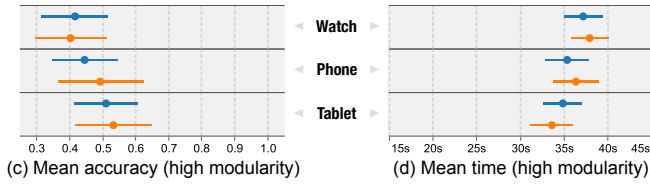
Figure 10. Node exploration task (T1) results of Study II. Error bars are 95% confidence intervals (CIs).
