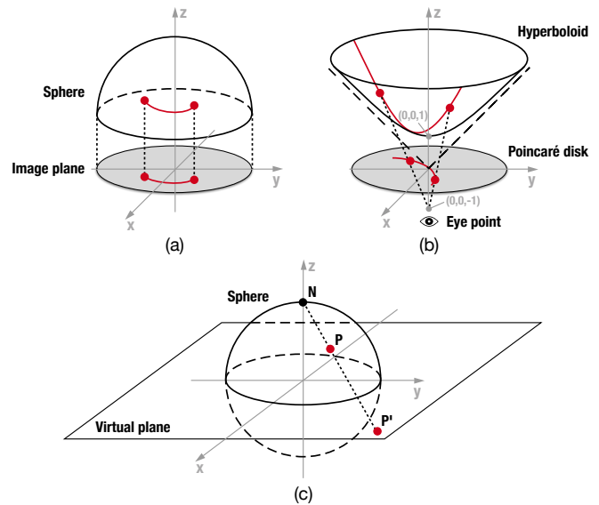
Figure 2. Illustrations of (a) the orthogonal projection from a sphere to a Euclidean plane, (b) the perspective projection from a hyperboloid surface to the Poincaré disk, and (c) the conformal mapping from the Riemann Sphere to a virtual plane.
