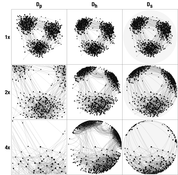
Figure 4. Illustrations of the zooming effect of D_p , D_h , and D_s . The graph contains 512 nodes and 4,096 links.
