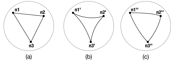
Figure 3. An illustration of a triangle displayed on (a) a Euclidean plane, (b) a Poincaré disk, and (c) a Riemann Sphere.
