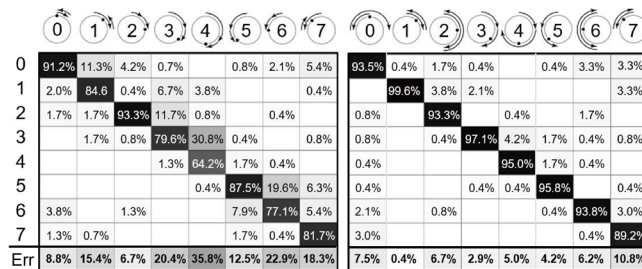
Figure 9. Confusion matrices for the DoublePoint (left) and VirtualPoint (right) techniques. Columns represent challenges and rows the participants' input.
