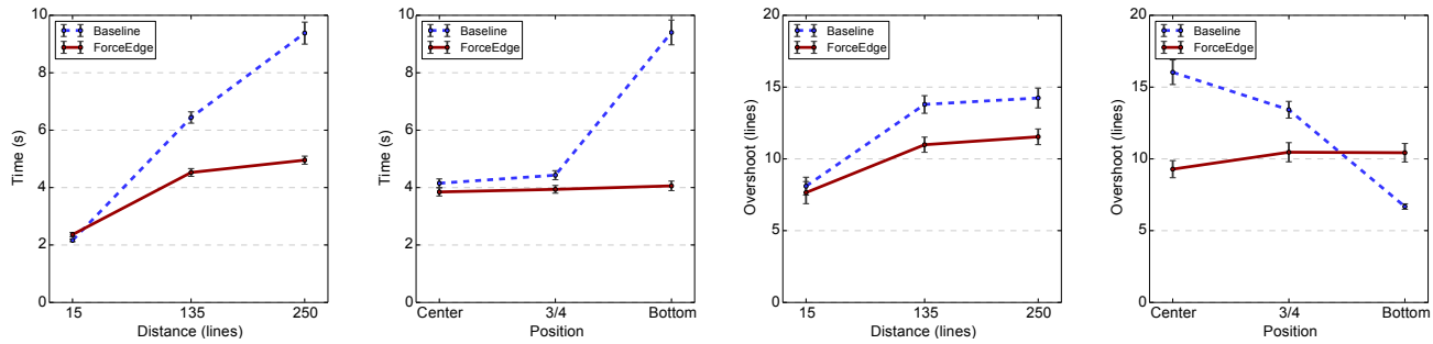
Figure 5: Results of study 2, from left to right: trial time (s) per distance, per position; overshoot (lines) per distance, per position
