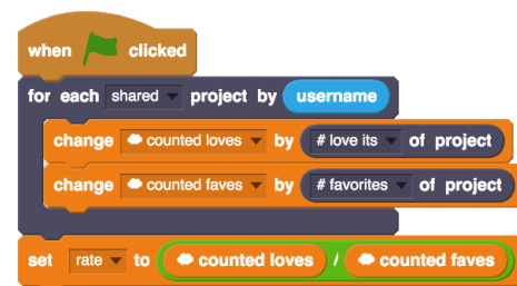
Figure 8: Code to store and analyze data from multiple user trajectories using persistent Cloud Variables (the ☁ icon beside the variable names indicates that it is a Cloud Variable).
