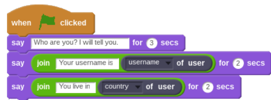
Figure 11: Code from user-created project that illustrates how the context-sensitive accessor block is incorrectly used.
