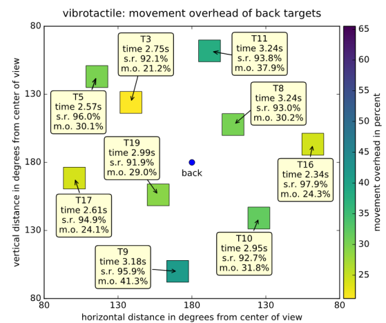
Figure 6. Vibrotactile condition, front (left) and back (right) targets: mean movement overhead (m.o.), median trial completion times and success rates (s.r.)
