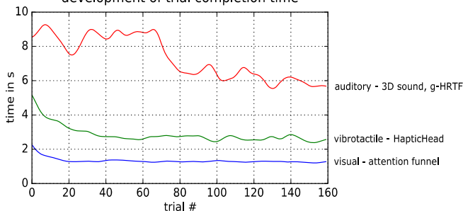
Figure 9. Average learning effect – time. Merged data, all participants. Curves: Gaussian weighted moving average (width=3, blue=visual, green=vibrotactile, red=auditory).
