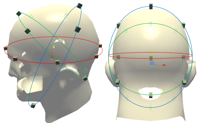
Figure 1. Placement of actuators in HapticHead. Note the three concentric ellipses around the user's head and no actuators close to the ear openings. The red ellipse contains 8 equidistant actuators, the green and blue ellipses each contain 6 actuators.
