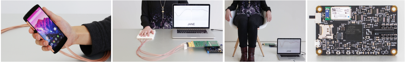
Figure 1. Zensei embeds implicit and uninterrupted user identification in mobile devices, furniture or the environment. Our custom, wide-spectrum multi-electrode sensing hardware allows high-speed wireless data collection of the electrical characteristics of users. A longitudinal 22-day experiment with 46 subjects experiment shows promising classification accuracy and low false acceptance rate. The miniaturized wireless Zensei sensor board (right) has a microprocessor, power management circuit, analog sensing circuit, and Bluetooth module, and is powered by a lithium polymer battery.
