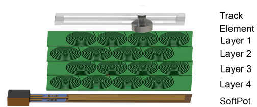
Figure 7: Exploded view of the PCB micro-coil system, consisting of a RTE, a linear track, flexible circuit layers containing interleaved electromagnetic coils, and a soft potentiometer.
