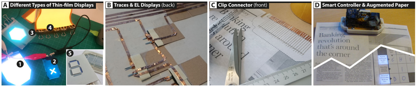
Figure 13. We considered several thin-film display technologies: cut (A1) & stenciled EL foils (A2), printed EL segments [46] (A3), elastomeric ELastoLite Panels® (A4) and printed EC SSDs [67] (A5). Finally, we used cut & stenciled EL foils in fast iterations. To realize paper traces we used combinations of copper (B) as well conductive tape with conductive ink (C). As a result, we came up with a 27 pin connector (C) for our smart clip (D).
