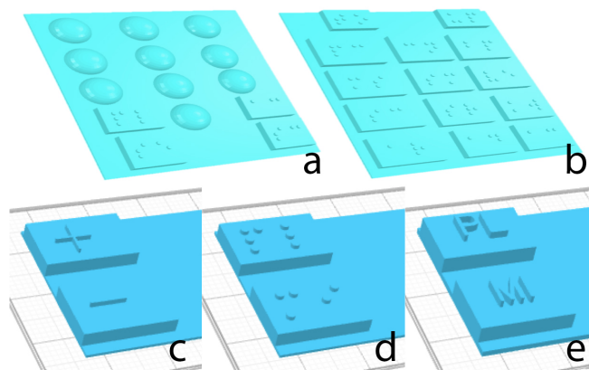
Figure 3. Shapes inform users of different functionalities. For example, half spherical buttons without Braille label indicates number buttons (a), while rectangular buttons with Braille labels indicate function buttons (b). Users are also able to change settings to use symbols (c), Braille (d), or embossed letters (e) for buttons labels such as plus and minus.
