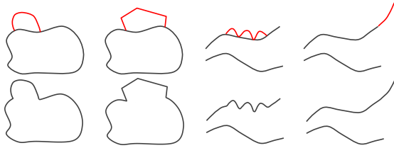
Figure 4. Overdrawing to modify profile and rail curves: (top row) over-drawn curves are shown in red, (bottom row) result of integrating over-drawn curves with profile and rail curves.
