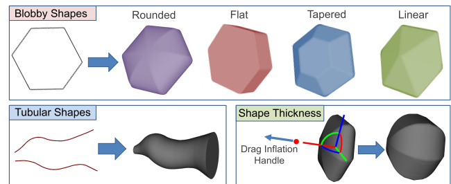
Figure 3. (top) Generating four types of blobby shapes from a profile curve; (bottom left) Generating a tubular shape from two rail curves; (bottom right) Increasing thickness or inflation magnitude of a blobby shape using the 3D manipulation widget.
