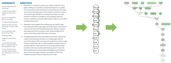
Figure 8: Parsing Process
