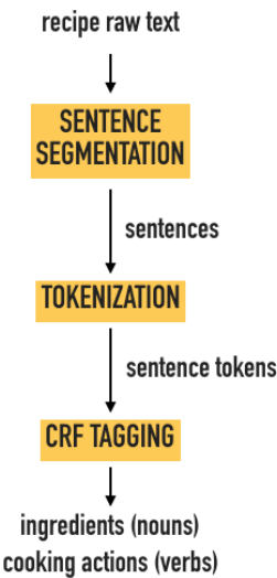
Figure 6: Pipeline
