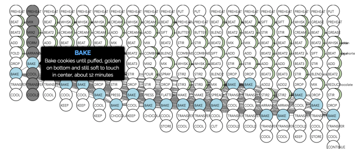
Figure 3: RecipeDeck
