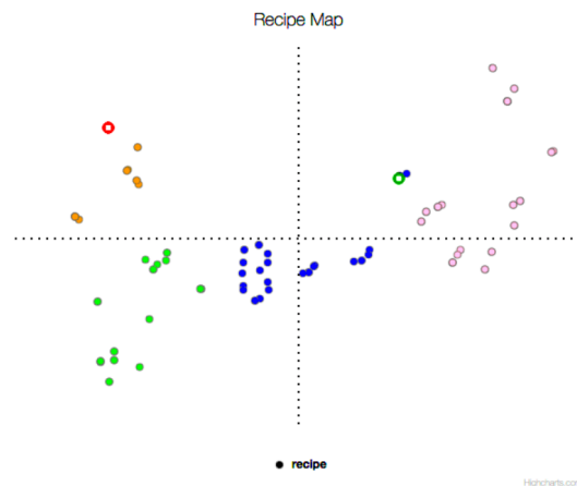
Figure 2: RecipeMap
