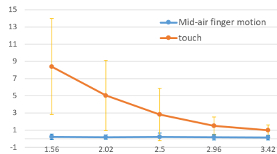
Figure 5. Mean and STD of miss-hits for 5 target sizes (vertical axis: number of miss-hits; horizontal axis: mm).
