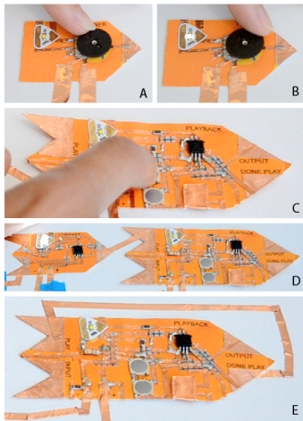
Figure 2: Adjusting tuner sticker with knob (A and B). Triggering playback with the onboard button (C), with an external signal (D) and with the Done Playing pin for repeating lopped playback (E)
