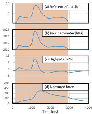
Figure 5: Response of the device when it was touched under the with-tape condition.
