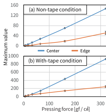
Figure 9: Force-sensitivity characteristic of each touch force: a) non-tape condition. b) with-tape condition.
