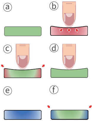
Figure 3: Changes of the air pressure inside the waterproof device. a) Before touch. b) Right after touch. c) During touch. d) A period of time after touch. e) Right after the finger leaves. f) Long after the finger leaves.
