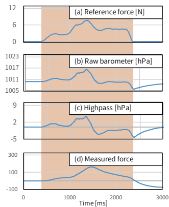
Figure 4: Response of the device when it was touched under the non-tape condition.
