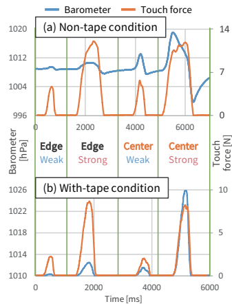
Figure 2: Waveforms of the air pressure and touch force in the waterproof device when it was touched at different touch positions and different touch forces. a) Non-tape condition. b) With-tape condition.
