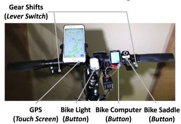
Figure 6: The study setup with existing mechanical inputs
