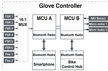
Figure 3: The schematic workflow of the prototype
