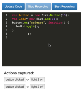
Figure 1: A Screen shot of Intuito's software showing the start recording, stop recording and update buttons, captured events and the generated output code.
