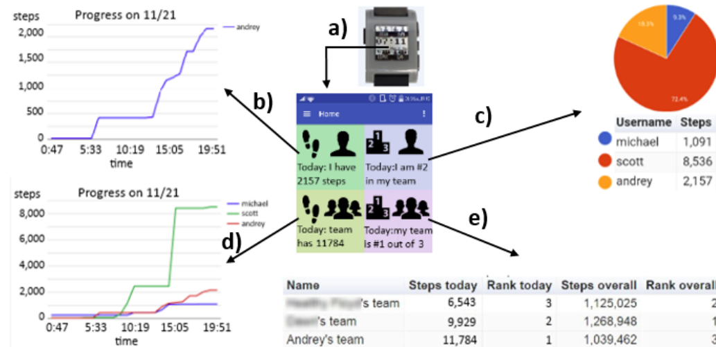
Figure 5: FitAware smartwatch watchface and the companion app interfaces explored. The elements on the watchface (a) directly map to the four squares on the Android app's home screen where tapping the top left square opens up a screen with the user progress chart ("my info") for the day (b). Tapping the top right square opens a visualization and table displaying each team member's contribution ("my rank") to the team steps (c). The bottom left opens up a progress chart ("team info") for all team members (d) and the bottom right square leads to a table with intervention statistics ("team rank") for the day and the whole period of the competition.
