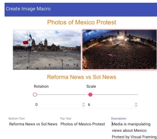
Figure 5: UnbiasedCrowd's Interface for creating an image macro using selected set of images.
