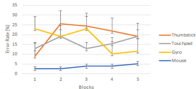
Figure 7: Error rate by block. Error bars show \pm 1 SD.
