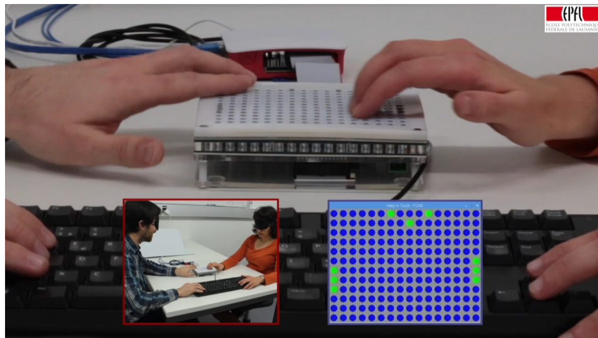
Figure 3: Tactile Pong, as an example of a serious game played on KiT. The two paddles can be seen as 3 raised taxels on the right and left edges, and the “ball” is under the fingers of the player on the right. The two raised taxels at the top are to keep score. The moving taxel vibrates to make it easier to track it as it moves across the display.
