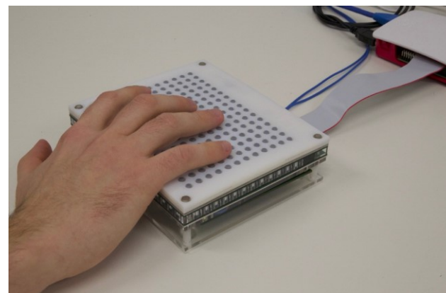
Figure 2: 12x16 haptic display (15 cm x 12.5 cm), and Raspberry Pi (top right). The user touches smooth plastic taxels, driven by an array of 192 high speed actuators.
