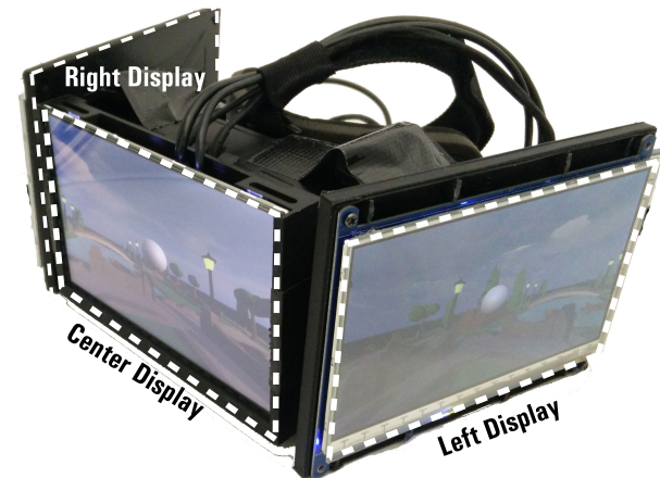
Figure 2: The hardware prototype of FaceDisplay, consisting of three touchscreens attached to the back and the sides of an Oculus Rift DK2.
