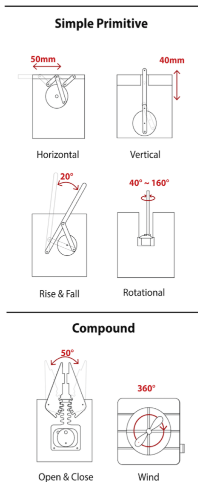
Figure 3: Motion Modules in Primitive Motions (horizontal, vertical, rotation) and Compound Motions (open & close)
