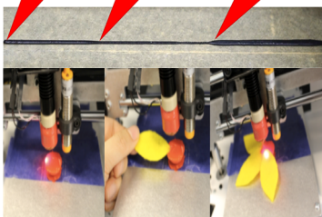
Figure 10. The connected a number of sensors enable the printer to control printing parameters, i.e. thickness of deposited lines real-time (Top). It can also guide human to enable inserting foreign items onto the object (bottom)
