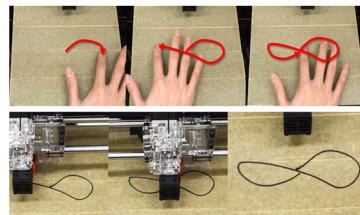
Figure 9. An early prototype of the Sensing Machine that captures users' gesture path and replicate 'drawing' with plastic. A leap motion tracks the human gesture, being connected to an Arduino to communicate with a 3D printer.
