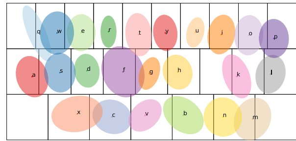
Figure 7: Touch point distribution in AGTex (95% confidence ellipses).
