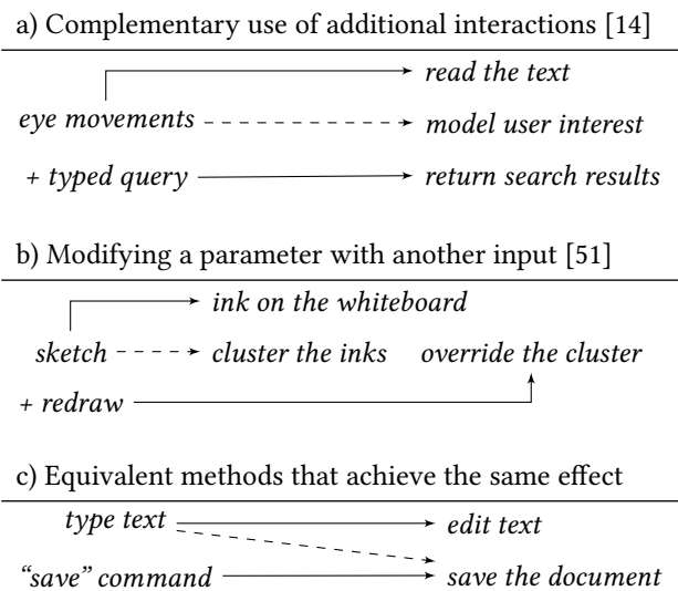
Figure 2: Diagrams showing an interaction that is designed to be implicit (dashed lines) within the context of other interactions.
