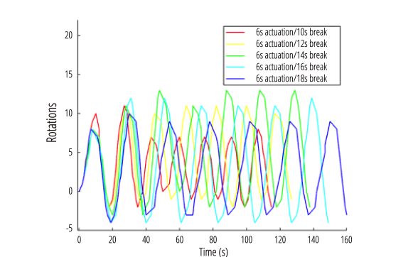
Figure 9: The number of rotations achieved by accumulated momentum according to different sets of actuation and break periods
