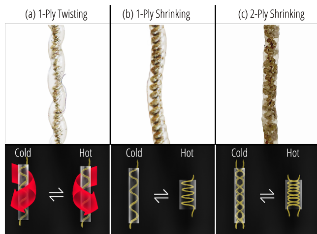
Figure 2: Actuation types and coiling shapes
