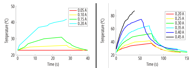
Figure 6: Temperature changes of thin actuator (left) and thick actuator (right) according to different currents.
