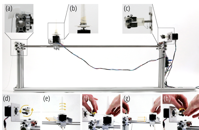
Figure 5: The process of making longer coils.
