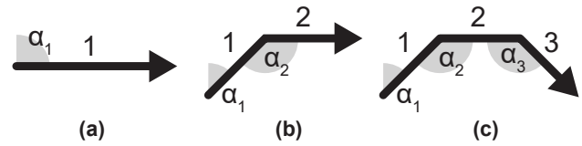
Figure 1: For one-segment gestures (a) we rotated \alpha_1 around 360° in 1° steps. For two-segment gestures (b) we rotated \alpha_1 around 360° and \alpha_2 from -90° to 90°, both in 15° steps. We rotated three-segment gestures (c) around 360° at \alpha_1 and from -90° to 90° at \alpha_2 as well as \alpha_3 , all three angles in 15° steps.
