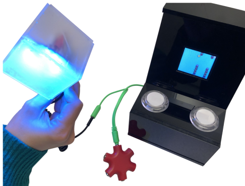
Figure 2. This custom designed accelerometer controller plugged into additional inputs using a headphone jack hub. This lets a user build their own controller and interactions for their game using MakerArcade.
