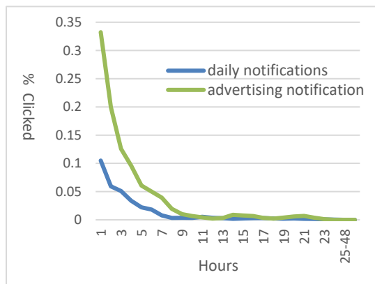
Figure 3: CTR as a function of number of hours since the notification was sent.
