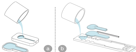
Figure 6: Casting process (a) for the inflatable chamber and (b) for the final unit.
