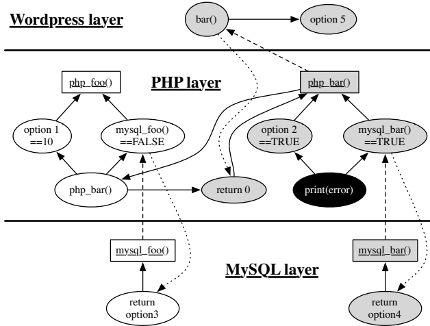
Figure 7: Cross-stack slice dependency graph for Figure 6. Solid lines indicate slice dependencies, dashed lines physical links and dotted lines slice dependencies derived from the physical links. The black node is the start node, while the white nodes could be ignored for optimization.
