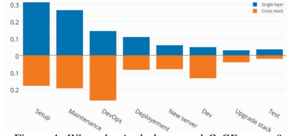
Figure 4: When do single-layer and CsCEs occur?
