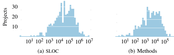
Figure 2. Histograms of projects size (bin width 0.15 on the log X-axis)
