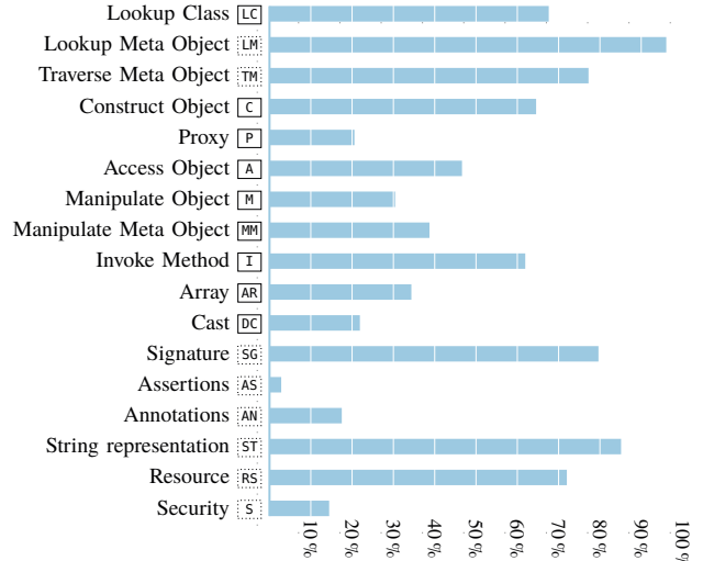
Figure 3. Reflection API usages, grouped per category (Table I), aggregated on project level, 17 projects (3.72%) contained no reflection. 356 projects (77.90%) contained at least one of the dynamic language features (□ categories).
