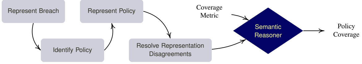
Fig. 3. SEMAVER methodology for determining policy coverage.
