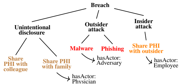
Fig. 1. Breach concepts. Lines represent subclass (is-a) relations among concepts. Arrows represent properties of concepts (has-a relations).
