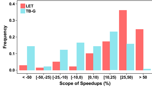
Fig. 3: Speedup distribution of LET
