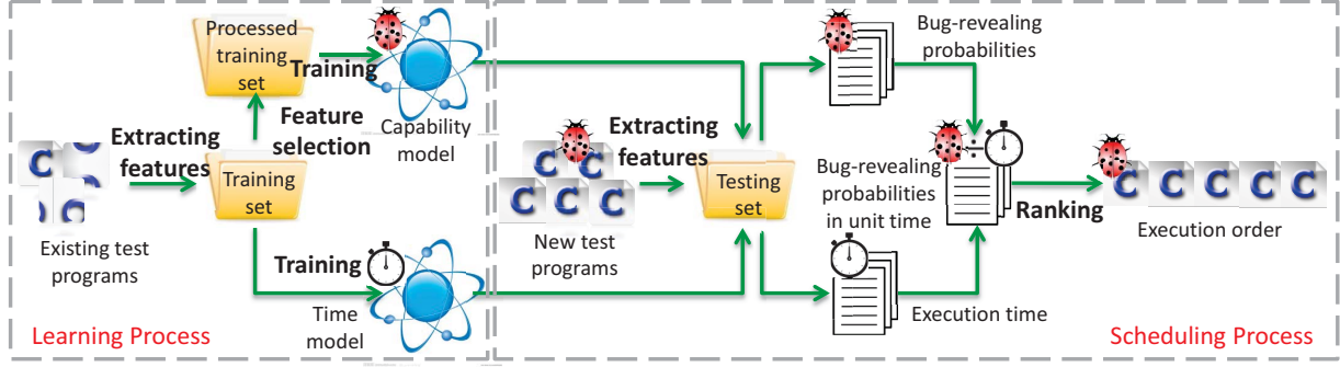
Fig. 1: Overview of LET
