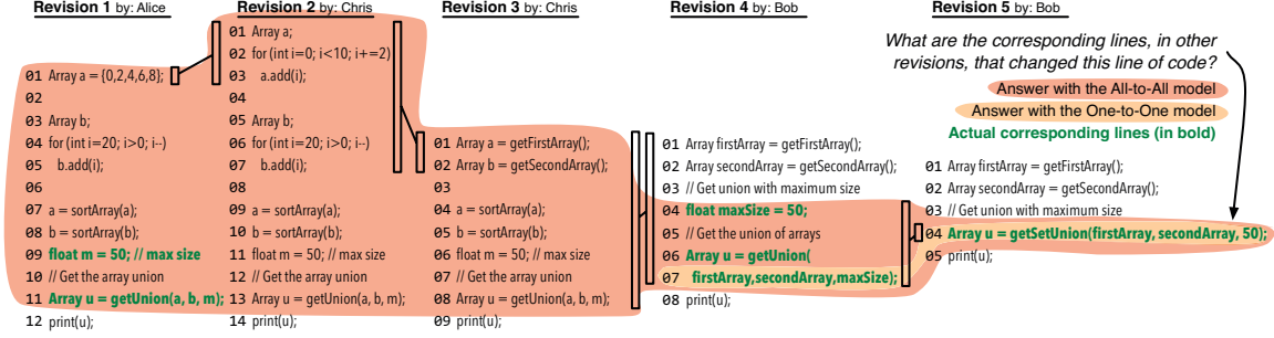
Fig. 1: Code evolution example
