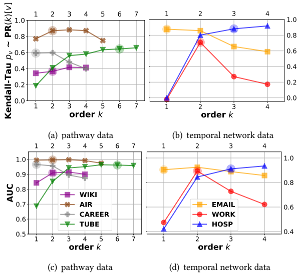
Figure 4: (a-b) show Kendall’s rank correlation between visitation frequencies p_v and PageRank (y-axis) calculated in k -th order model for different k (x-axis) in pathways (a) and temporal networks (b). (c-d) show Area Under Curve (AUC) for prediction of 15% most frequently visited vertices based on PageRank computed for different k . Values k that correspond to the detected order K_{opt} are highlighted (cf. Table 1).
