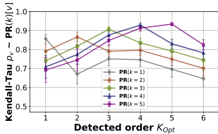
Figure 3: Kendall’s rank correlation between k -th order PageRank PR(k) and ground truth vertex visitation frequencies p_v (y-axis) in paths with different detected orders K_{opt} (x-axis). Results are averages of 100 runs, fitting a multi-order model to N = 20000 synthetically generated paths of length L = 10 in random graphs with 100 vertices and 350 edges. Error bars indicate standard deviation.
