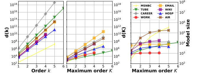
Figure 5: Degrees of freedom in standard k -th order Markov chain (left) and multi-order graphical models (middle) for empirical data. Right panel: actual size of multi-order models, using sparse representations of transition matrices.
