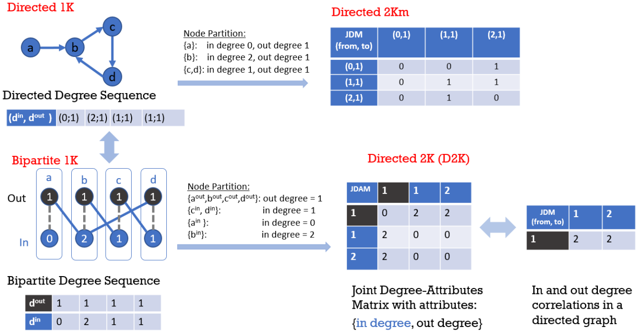
Figure 1: Defining Directed 2K, to capture degree correlations in a directed graph. Top left, Directed 1K : Directed graph with a given degree sequence (DDS). Bottom left, Bipartite 1K : Mapping of the previous to a Bipartite undirected graph with a given bipartite degree sequence; non-chords in the bipartite graph (shown in dashed line) correspond to self-loops in the directed graph. Bottom right, Directed 2K (D2K) : Joint-Degree-Attribute Matrix (JDAM), where nodes of the bipartite graph are partitioned by their degree-and-(in or out) attribute or equivalently the in and out degree correlations of the directed graph. Top right: Directed 2Km : Joint Degree Matrix (JDM) for directed graphs, where nodes are partitioned according to their (in degree, out degree).
