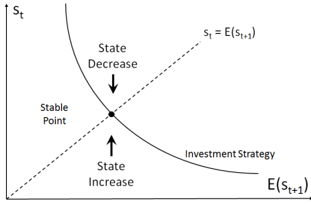
Figure 3: Three Scenarios of an Investment Strategy
