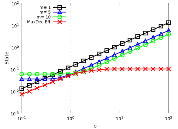
Figure 10: Impact of Noise in Simulation
