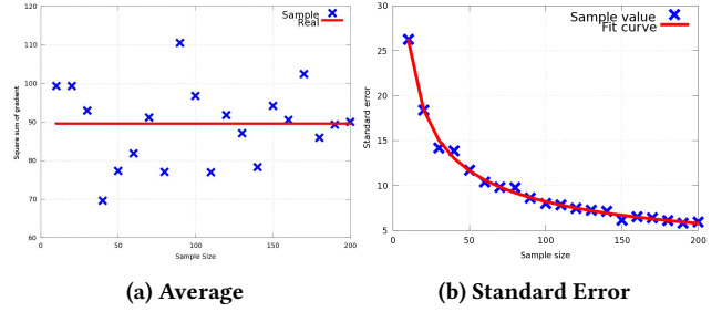
Figure 6: Impact of Sample Size
