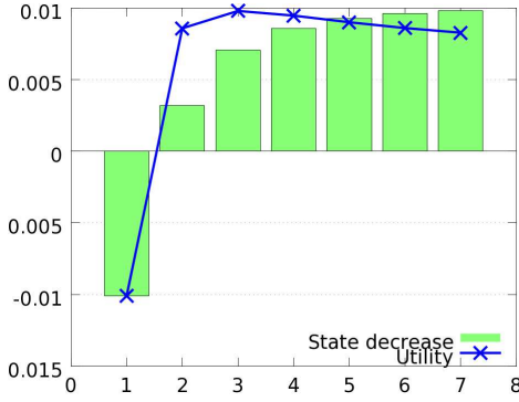
Figure 4: State decrease & Utility of different investment m
