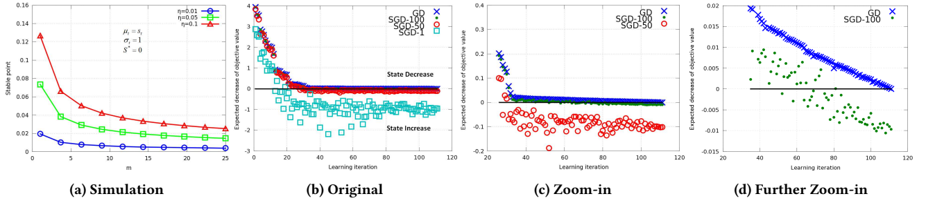
Figure 7: Verification of Stable Point for SGD. The x -axis represents the learning iterations of gradient descent (GD). The y -axis represents the decrease of objective value for a single iteration.
