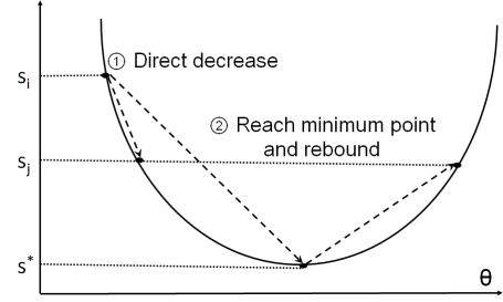
Figure 1: Illustration of State Transfer in Learning
