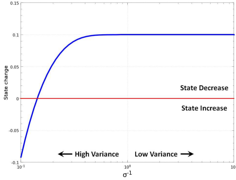
Figure 2: Correlation between State Change s_t - E_m^{s_t}(s_{t+1}) and Variance \sigma_t^2 . Note that the x-axis is \sigma^{-1} .
