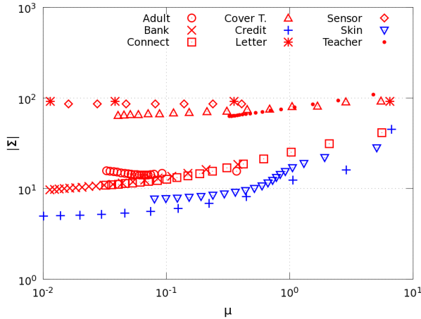
Figure 9: Noise Demonstration in Real Data
