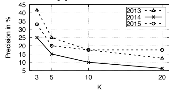
Figure 5: Precision of top K MARAS MDAR signals.
