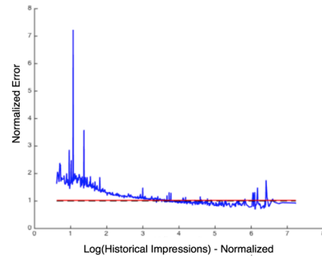
Figure 2: We show how the click-model’s accuracy behaves as a function of the historical impressions received by corresponding creative. On the x-axis is the logarithm of the number of historical impressions (normalized for position effects, and rescaled), and the y-axis is a notion of error called the relative bias of the ad. We see that for cold ads, the error is substantially worse than for warm ads.
