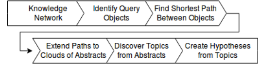
Figure 3: MOLIERY query pipeline.
