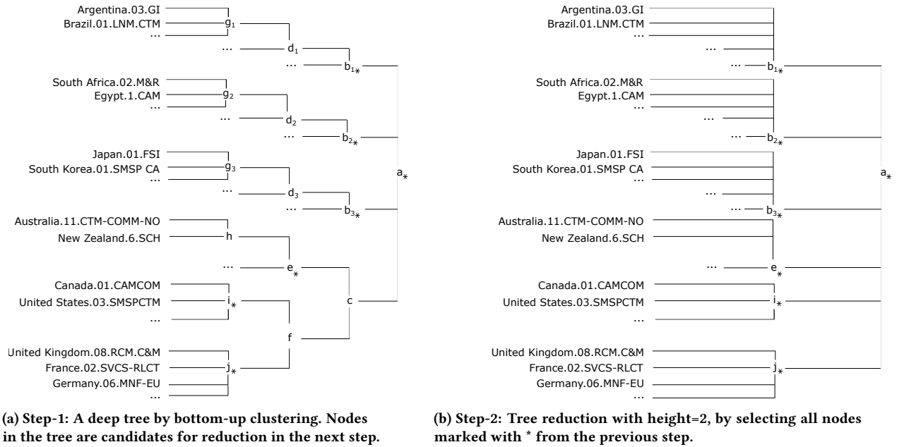
Figure 1: Illustration of the two steps in our approach using an enterprise concept called ATU (account team unit) specific to this spreadsheet corpus. Some values are slightly redacted for anonymization.
