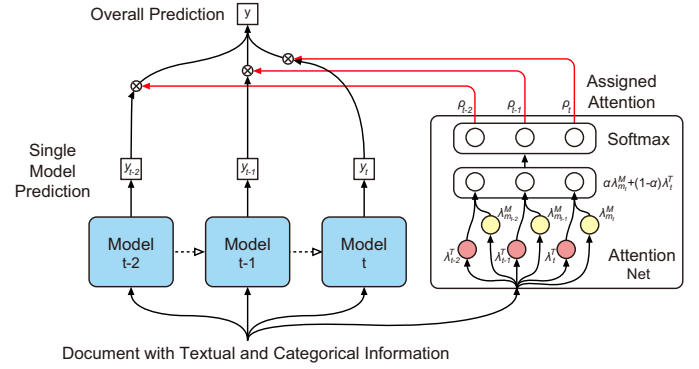
Figure 3: Dynamic attention over multiple deep nets.
