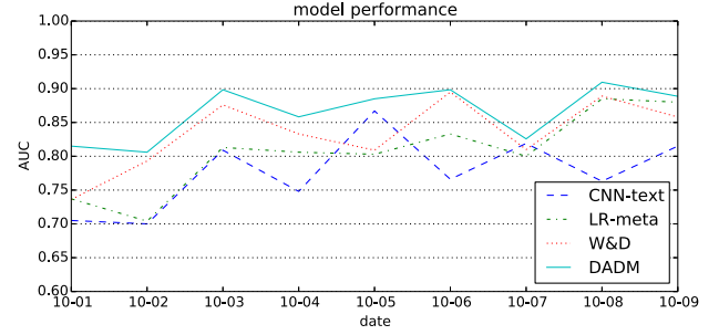
Figure 6: AUC performance of quality article recommendation over 9 days (Oct. 1-9, 2016).
