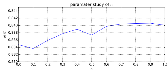
Figure 8: AUC performance against \alpha in Eq. (6).
