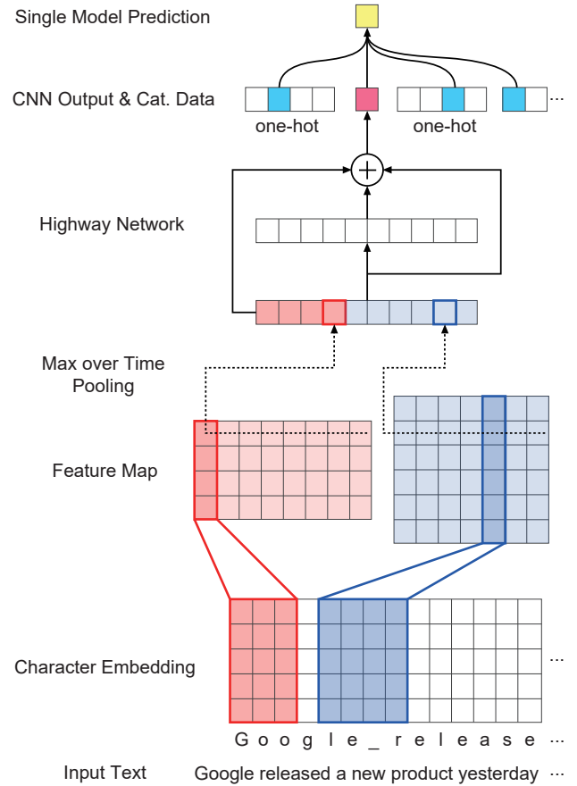
Figure 2: CNN architecture for text prediction.
