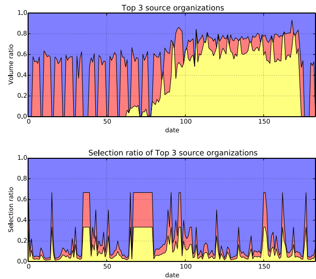
Figure 5: Dynamic characteristics of 3 main source organizations. Each of the 3 areas in the figures represents the proportion of their total volume (above) and selected articles (below).
