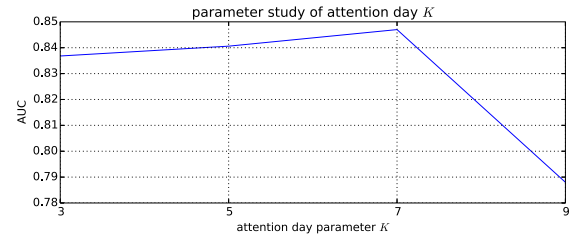
Figure 7: AUC performance against the number of attention days of DADM.
