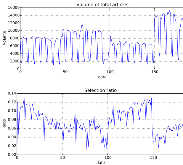
Figure 4: Dynamic characteristics of the dataset. Above: The change of the number of total submitted articles over time. Below: The change of the editors’ selection ratio over time.
