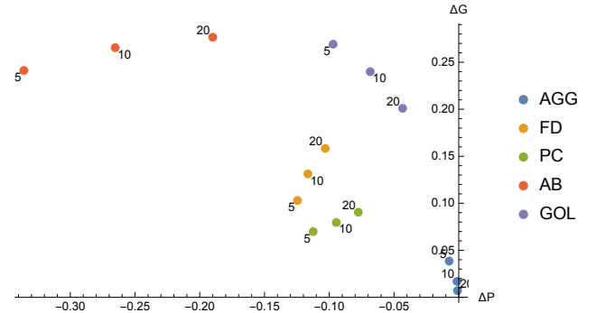
Figure 2: The change in the Gini index and the precision of the diversified solutions when the recommendation list length is varied. Values to the right and towards the top are better.
