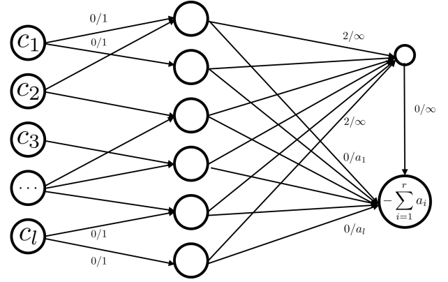
Figure 1: The network flow model for the MIN-DISCREPANCY problem with nodes labelled with their supply and arcs labeled with their cost/capacity. Unlabelled nodes have zero supply. much as \deg_G^+(u_i) \geq c_i flow to the sink t_2 via any c_i different neighbors. Note that there are |E| + 2|R| + 1 arcs in total in our flow network. The complete flow network constructed this way is shown in Figure 1.
