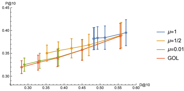
Figure 3: Precision discrepancy trade-off in the MovieLens-1m dataset using the MF recommender. In each series, the number of edges in the input graph increases towards the left.
