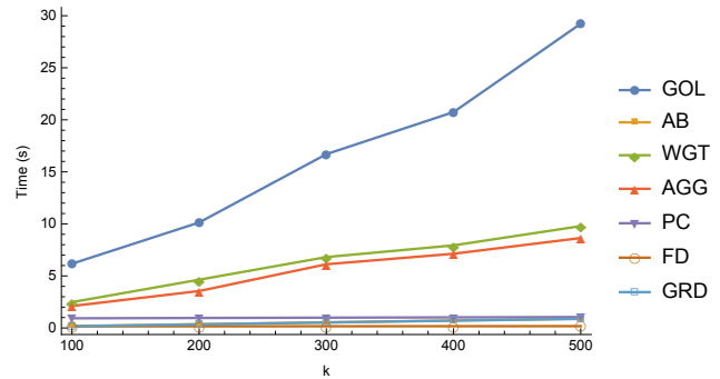
Figure 4: Time to optimize the top-10 recommendation task in MovieLens-1m based graphs in seconds ( |L|=5800, |R|=3600 )
